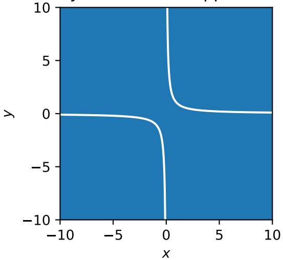
xy \neq 1 : Second approach
