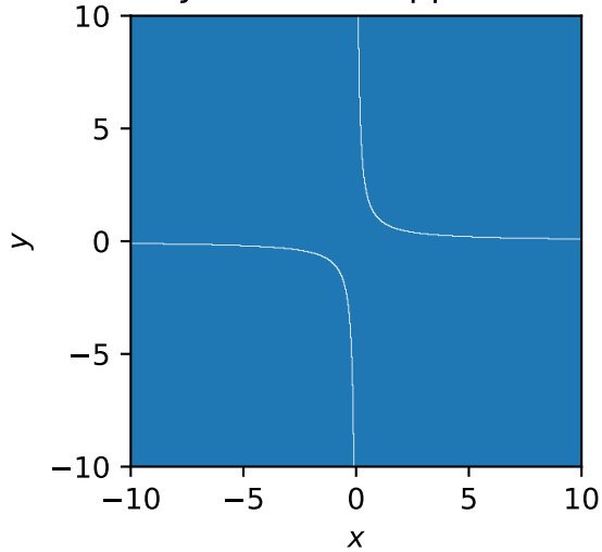
xy \neq 1 : First approach
