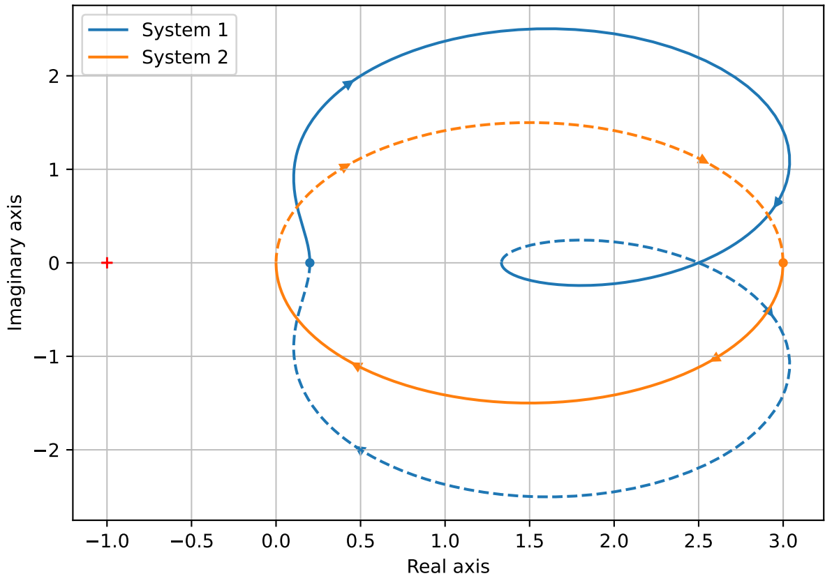
Nyquist Plot
