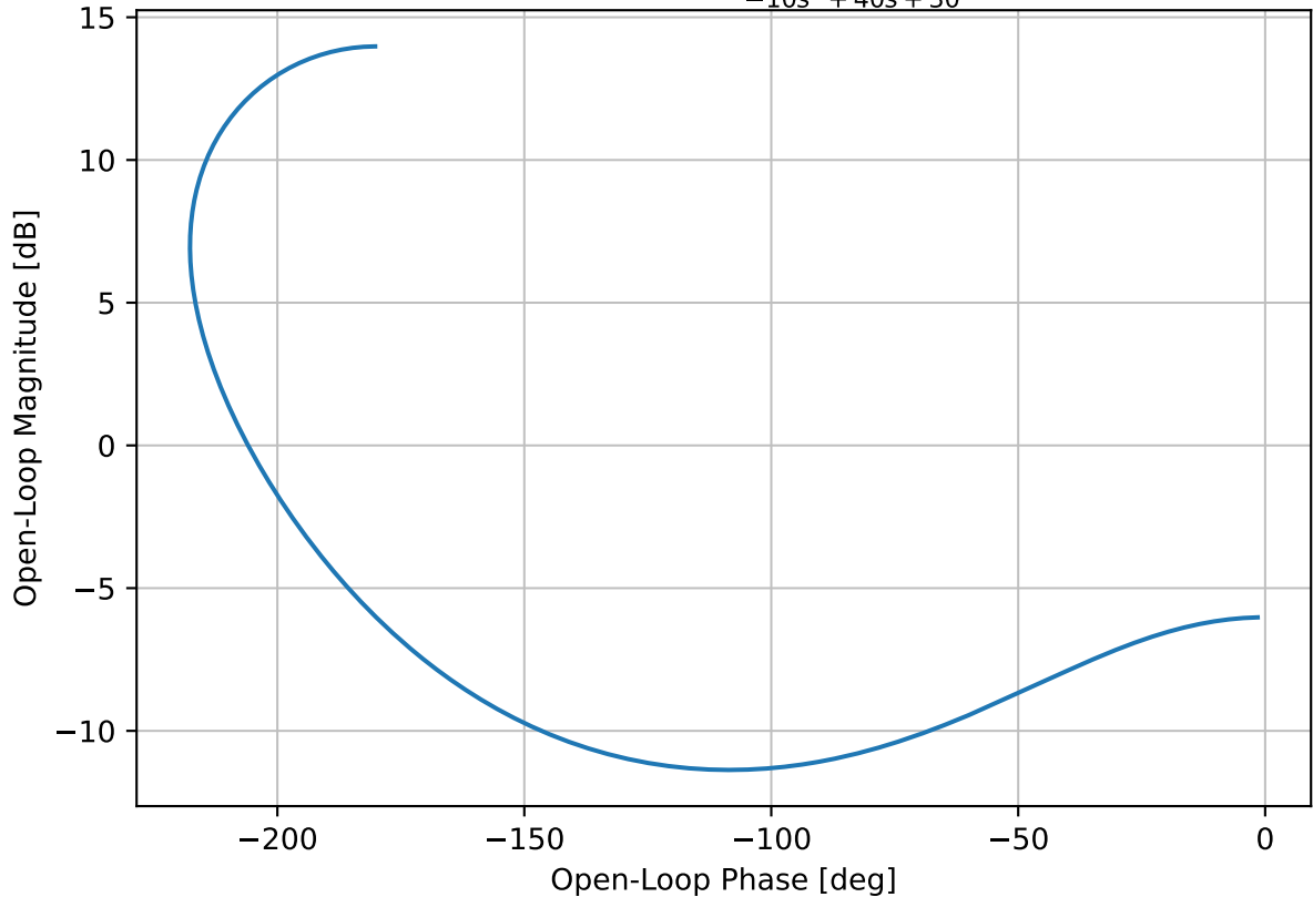
Nichols Plot of \frac{50s^2 - 20s + 15}{-10s^2 + 40s + 30}
