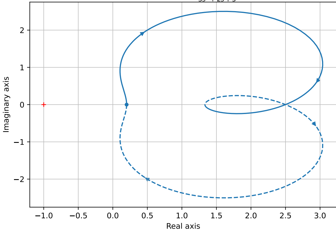
Nyquist Plot of \frac{4s^2 + 5s + 1}{3s^2 + 2s + 5}
